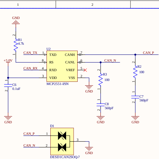
CAN Bus
