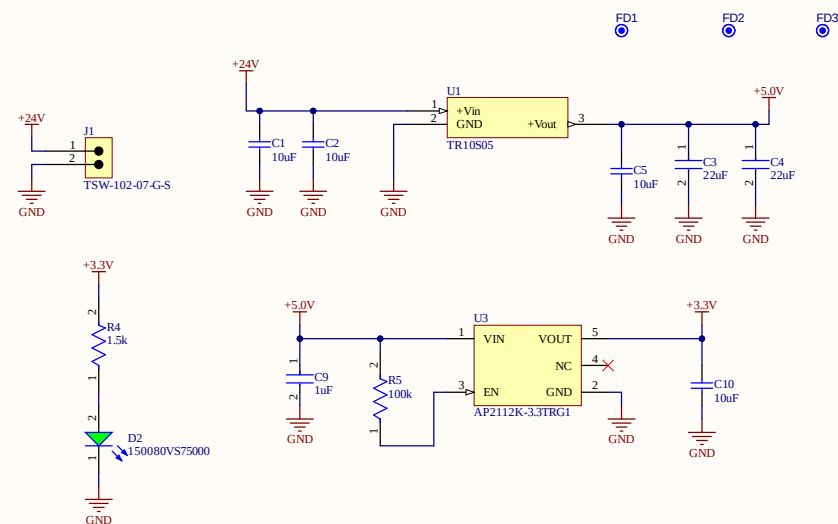
Power
