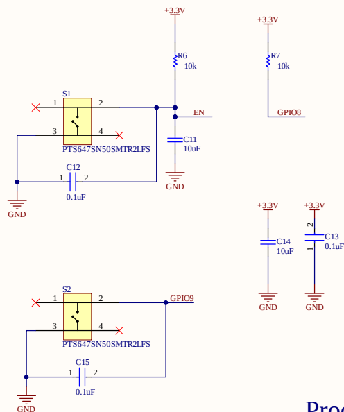
Processor
